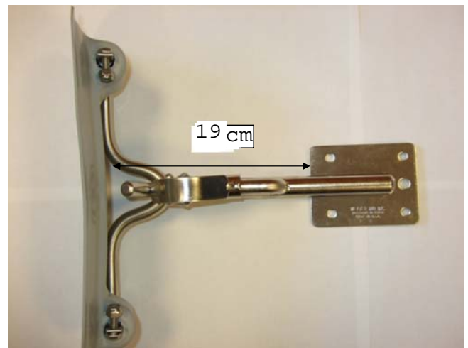
RDB100 - 6" Extended Davit
